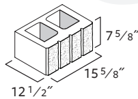
12x8x16 Stretcher Oversized
