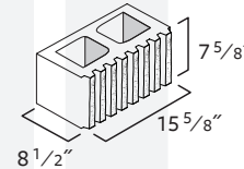
8x8x16 Stretcher Oversized
