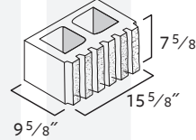
10x8x16 Stretcher
