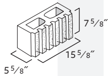
6x8x16 Stretcher Oversized
