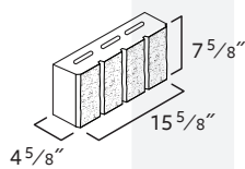
4x8x16 Cored Stretcher Oversized
