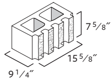
9 1/4" Stretcher Oversized
