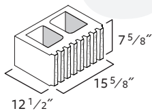
12x8x16 Stretcher Oversized
