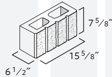
6x8x16 Stretcher Oversized
